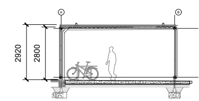
PROPOSED SECTION SCALE 1:200
