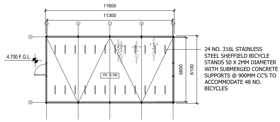
PROPOSED GROUND FLOOR PLAN SCALE 1:200
