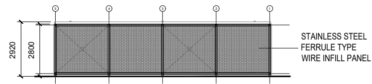
PROPOSED WEST ELEVATION SCALE 1:200
